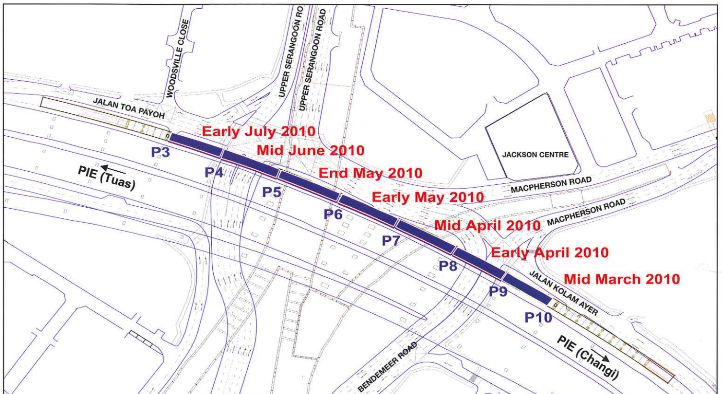
Proposed schedule for the launching of precast concrete beams at Woodsville Interchange
